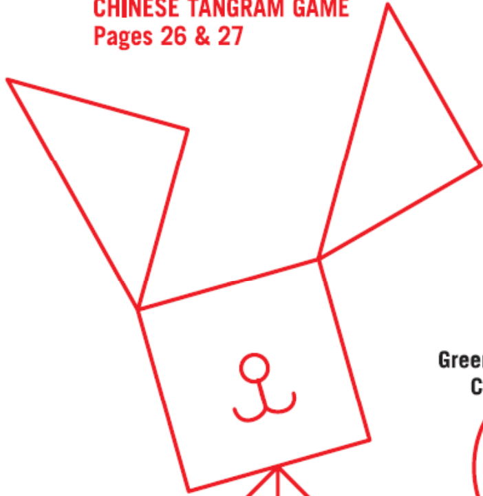
Rabbit tangram
